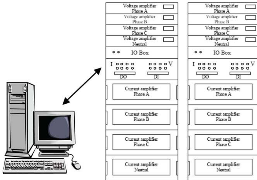
Figure 1. Two-terminal laboratory set-up
