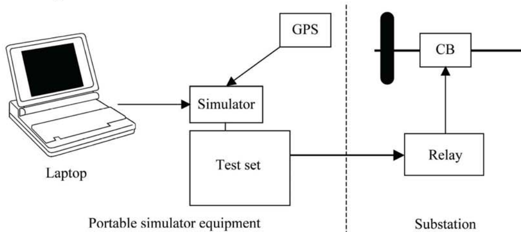
Figure 2. Portable simulator setup
