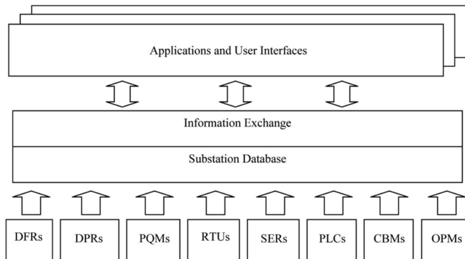
Figure 4. Data sources in a substation automation system
