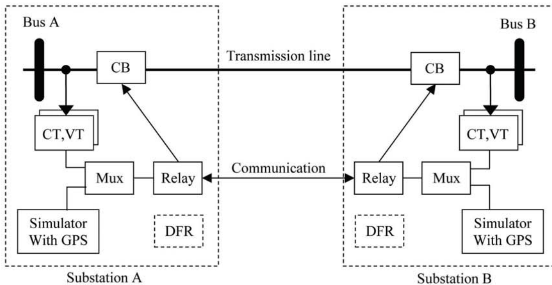
Figure 3. Digital simulator permanently installed in substations
